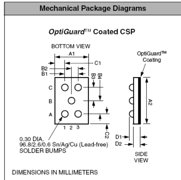
Package Dimensions for CM1204 Chip Scale Package
