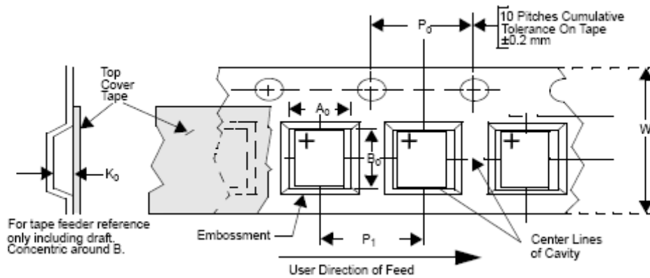
Figure 5. Tape and Reel Mechanical Data
